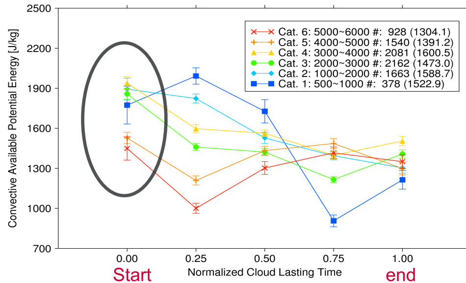
From Zhanqing Li, based on the data from Varble2018
